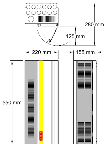
SCH1210 D version - 690x220x155mm RCBO & RCBOX version - 550x255x155mm
